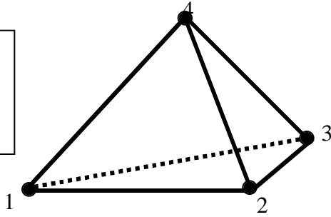
CONTINUUM THREE-D ELEMENT C3D4: 4-NODE LINEAR TETRAHEDRON
