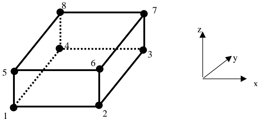
CONTINUUM THREE-D ELEMENT C3D8: 8-NODE HEXAHEDRON (BRICK)
