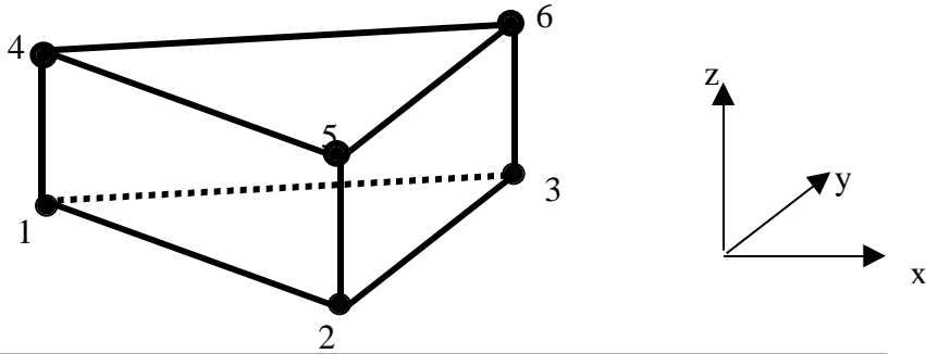
CONTINUUM THREE-D ELEMENT C3D6: 6-NODE LINEAR TRIANGULAR PRISM
